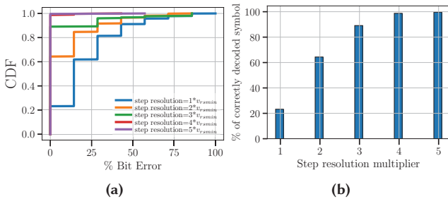
Figure 16: a) shows how the percentage bit error improves as we increase the step resolution of the voltage encoder. With step resolution, 5 * v_{r_s} = 11.81 mV, we can correctly decode 99% of the sent symbols.
