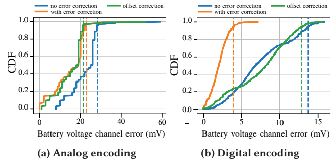
Figure 13: CDF of the error in received battery voltage. The channel error is significantly reduced after calibration using the proposed error correction technique. The dash lines correspond to 95th percentile error values.
